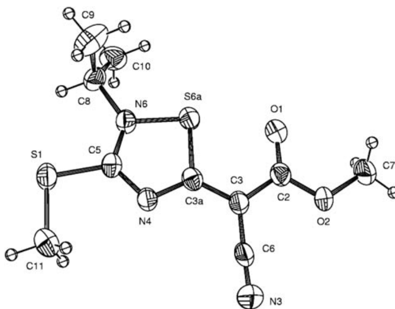
FIGURE 1 Solid-state molecular structure of 16a . Selected bond lengths ( \text{\AA} ): N6–C5 1.326 (8), C5–N4 1.331 (7), N4–C3a 1.344 (8), C3a–S6a 1.746 (6), S6a–N6 1.724 (5), C3a–C3 1.394 (8), C3–C2 1.422 (8), C2–O1 1.228 (7), O1–S6a 2.395 (5). Selected bond angles ( ^\circ ): N6–C5–N4 117.5 (5), C5–N4–C3a 109.4 (5), N4–C3a–S6a 114.4 (4), C3a–S6a–N6 87.2 (3), S6a–N6–C5 111.4 (4), S6a–C3a–C3 119.0 (4), C3a–C3–C2 117.2 (5), C3–C2–O1 121.9 (6), N4–C3a–C3 126.6 (5), O1–S6a–N6 167.5 (3); dihedral angle (N6–C5–N3–C3a–S6a/O1–C2–C3–C3a–S6a) 0.8(3)^\circ .
